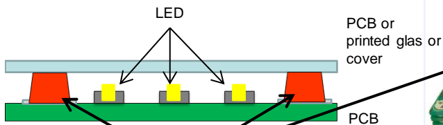
Abatek SMT Damper-Spacer
