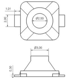
SMT Silicone Key on PCB
